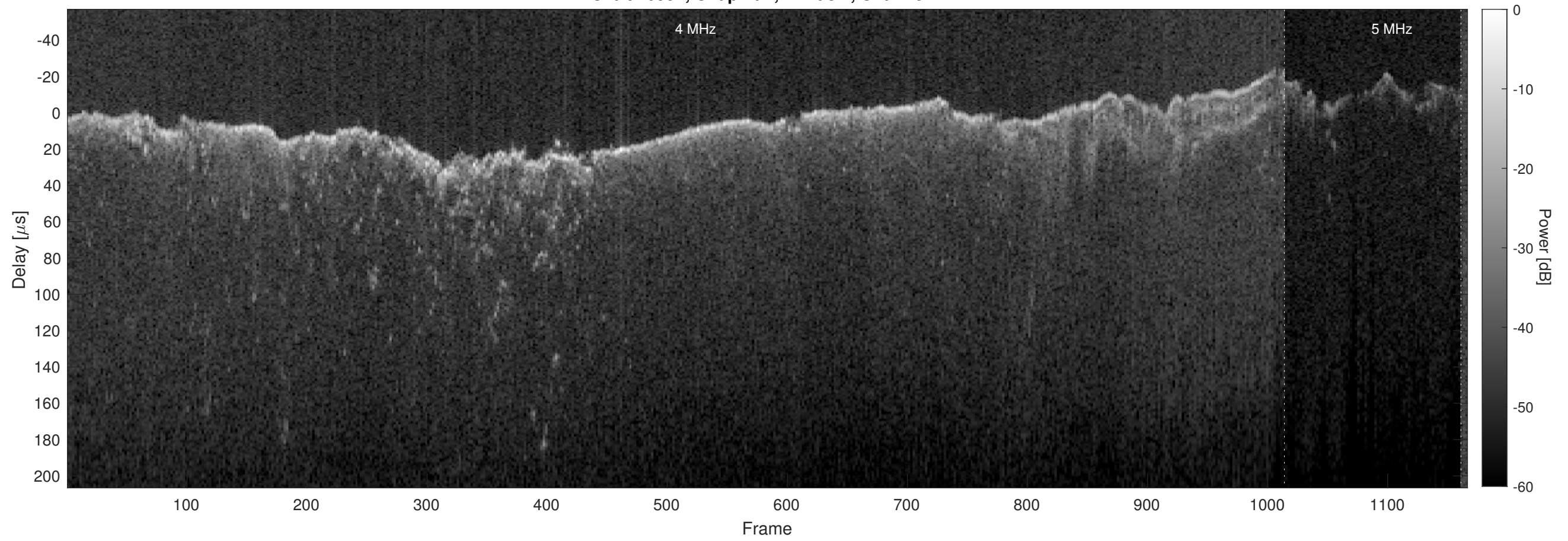
Orbit 10994, Chapman, Window, Channel 2
