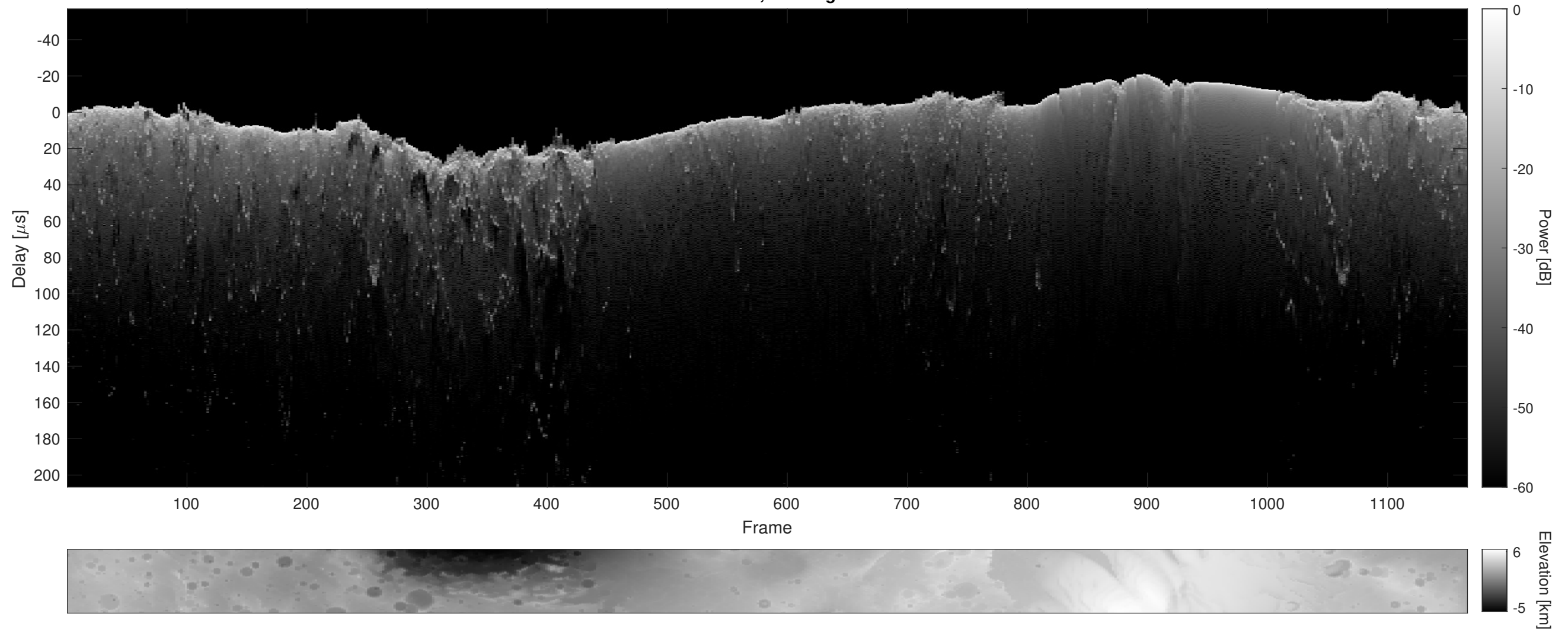
Orbit 10994, Cluttergram
