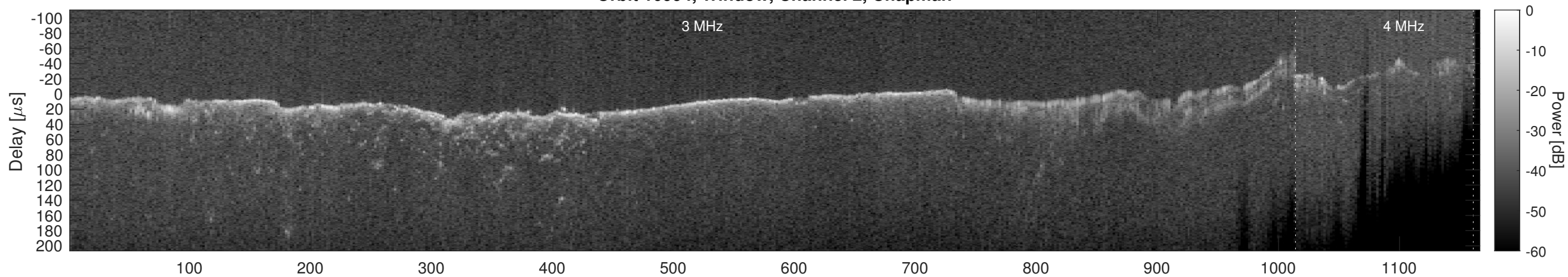
Orbit 10994, Window, Channel 2, Optimized
