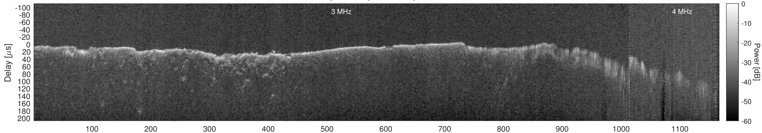
Orbit 10994, Window, Channel 2, Chapman
