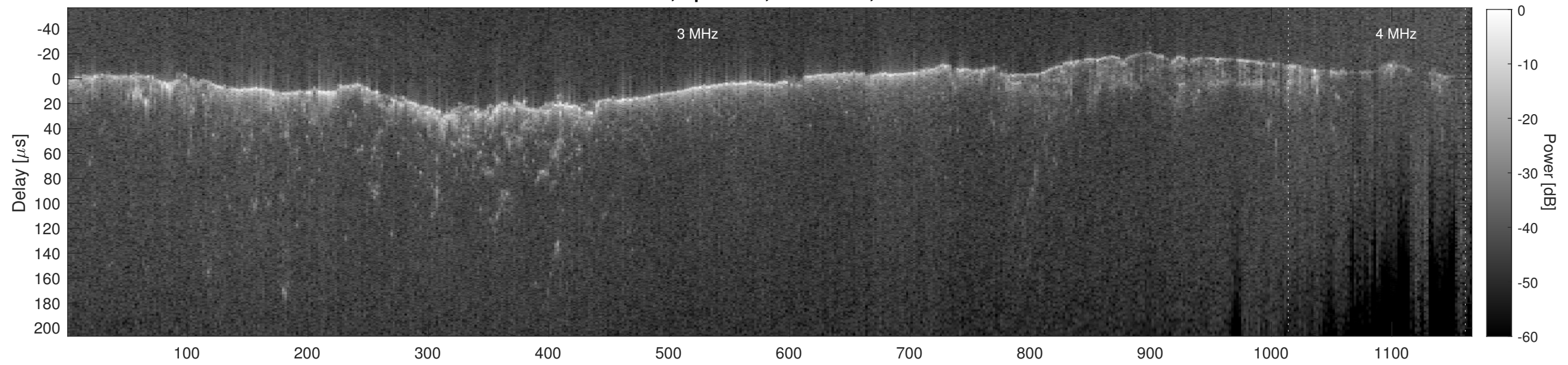
Orbit 10994, Cluttergram
