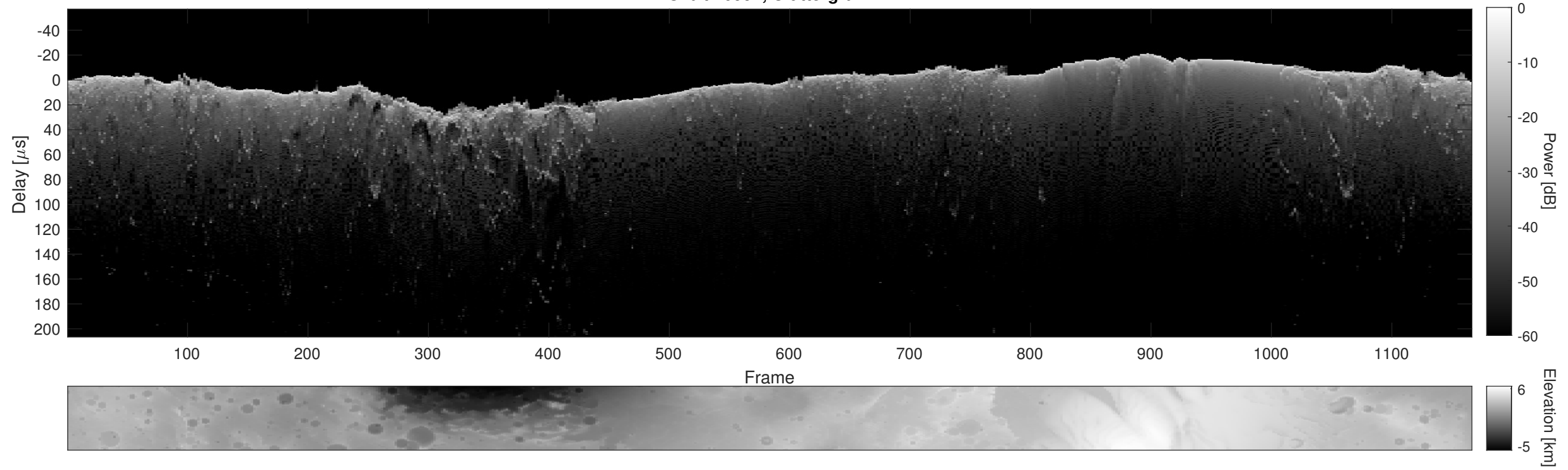
Orbit 10994, Cluttergram
