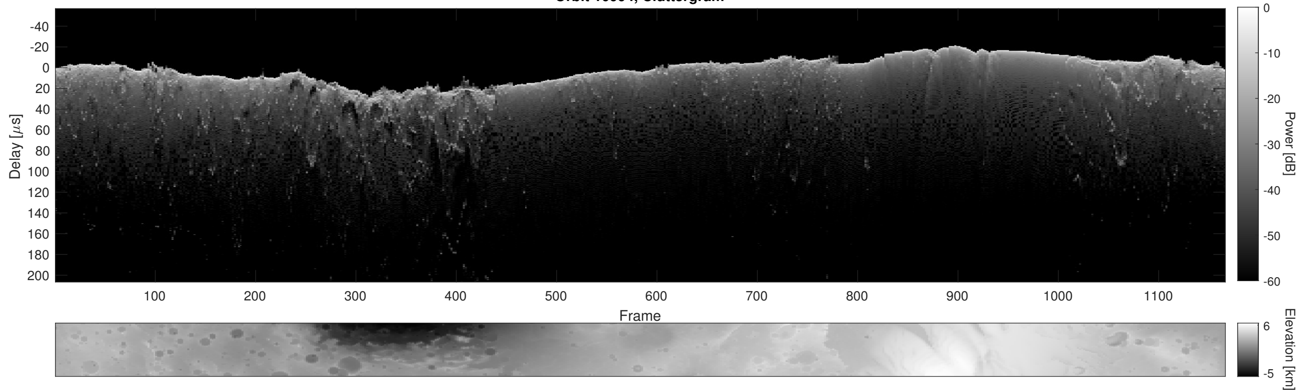
Orbit 10994, Cluttergram
