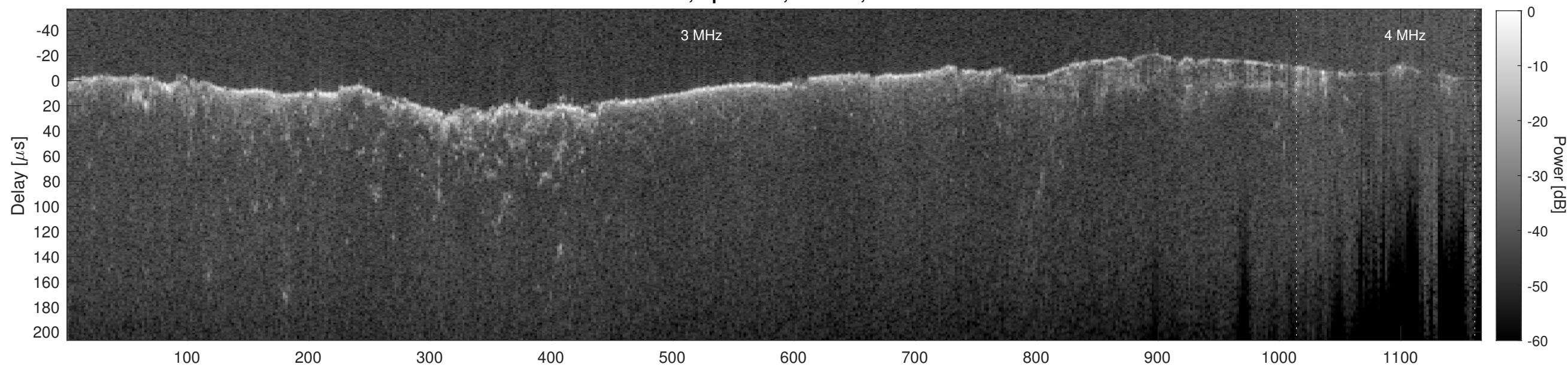
Orbit 10994, Cluttergram
