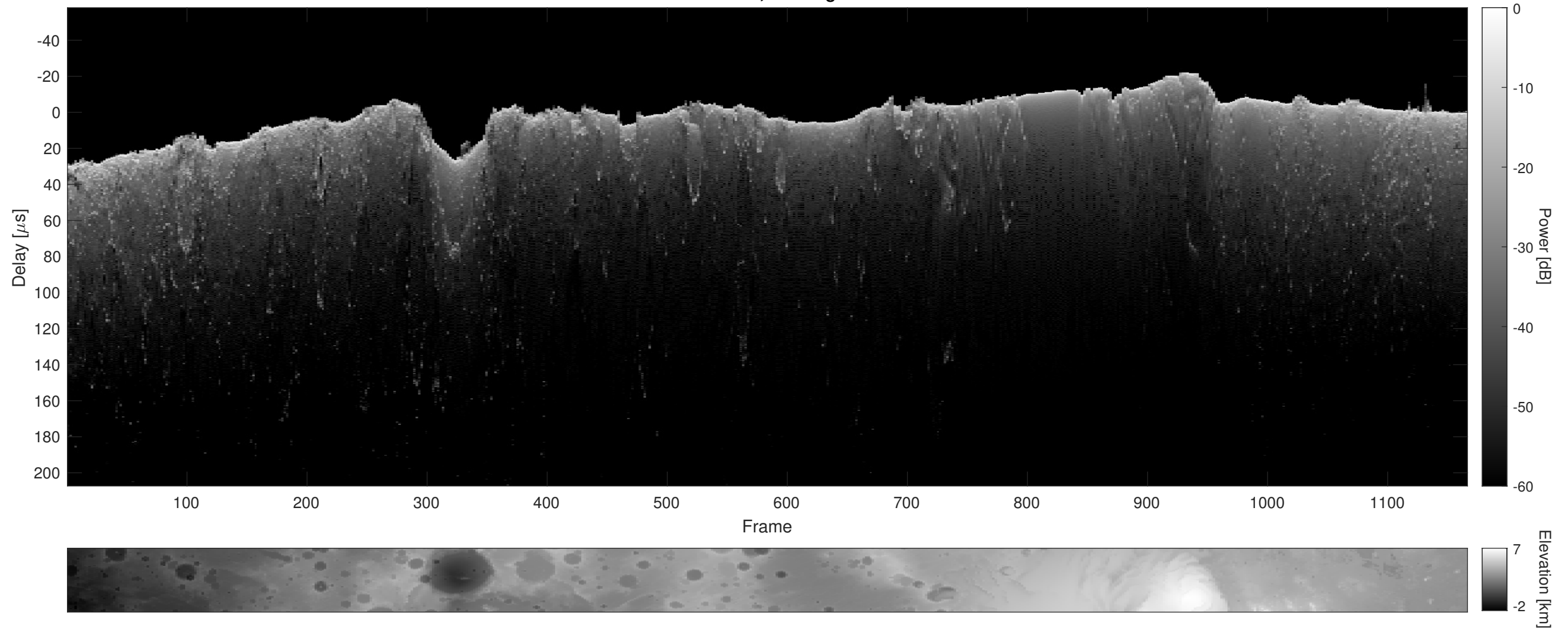
Orbit 10996, Cluttergram
