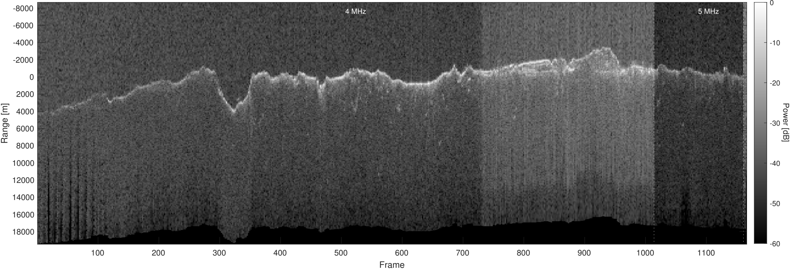
Orbit 10996, Optimized, Window, Depth-Corrected, Channel 2
