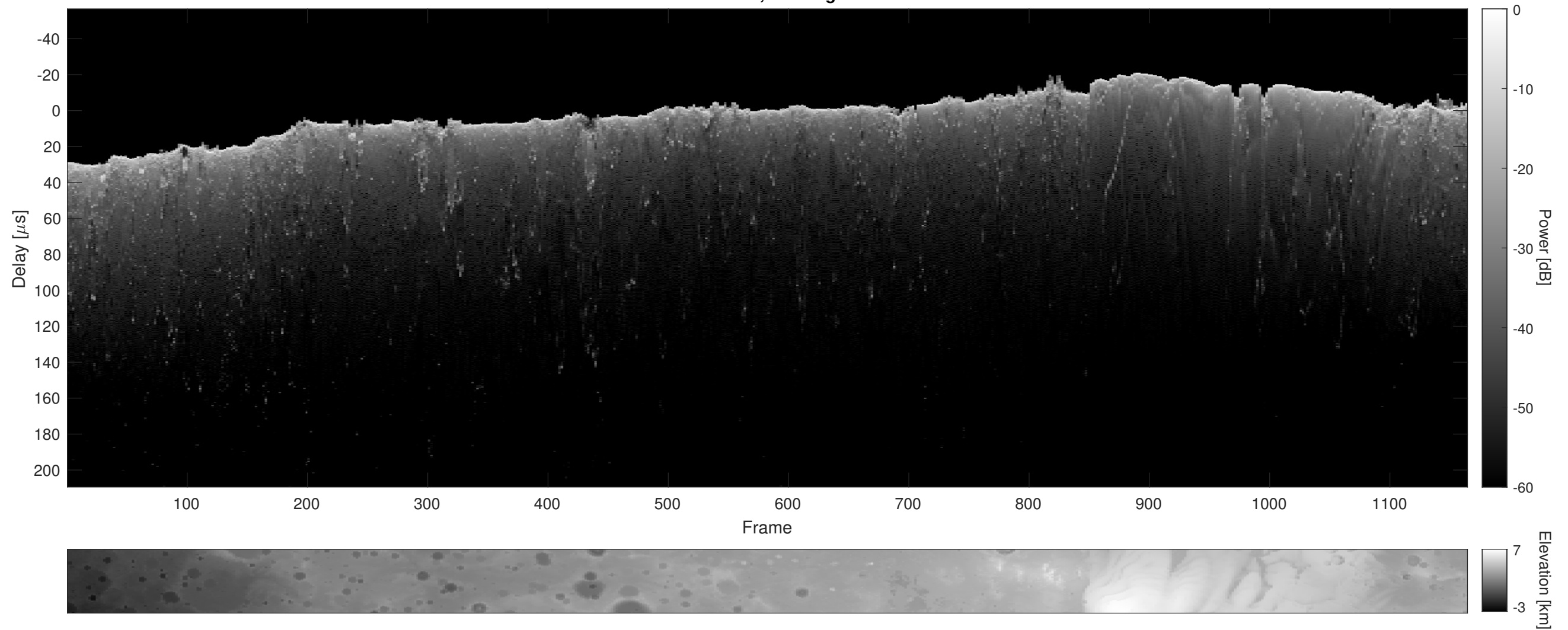
Orbit 10998, Cluttergram
