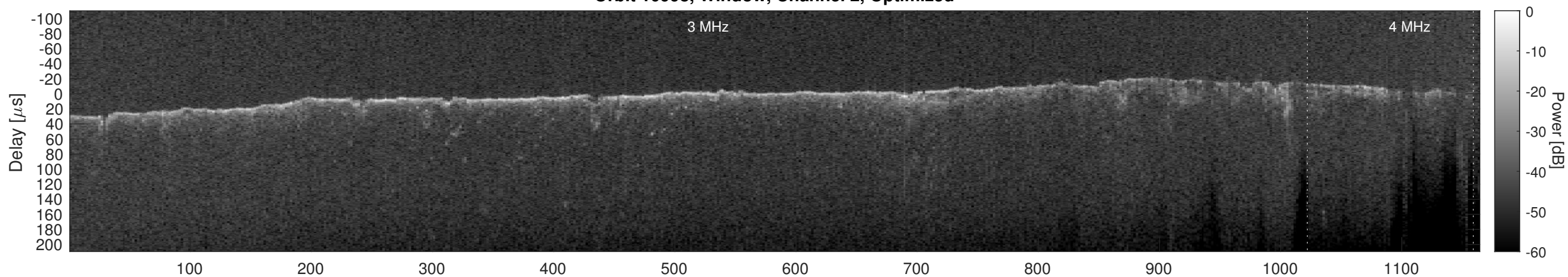
Orbit 10998, Cluttergram
