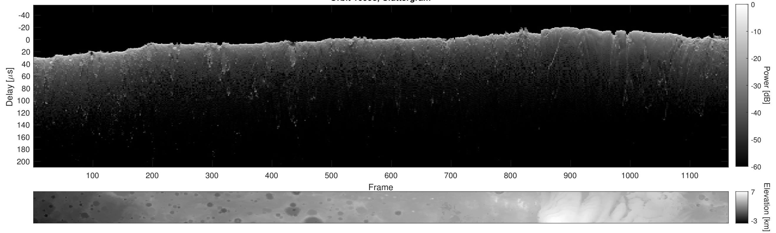
Orbit 10998, Cluttergram
