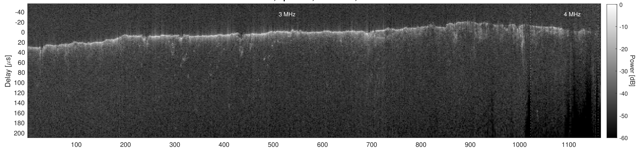
Orbit 10998, Cluttergram
