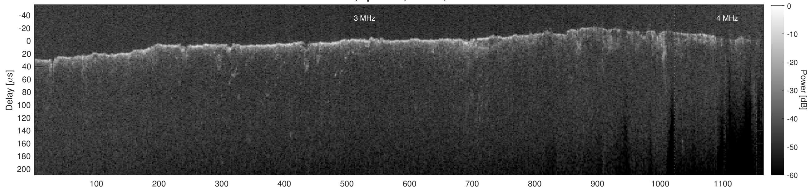
Orbit 10998, Cluttergram
