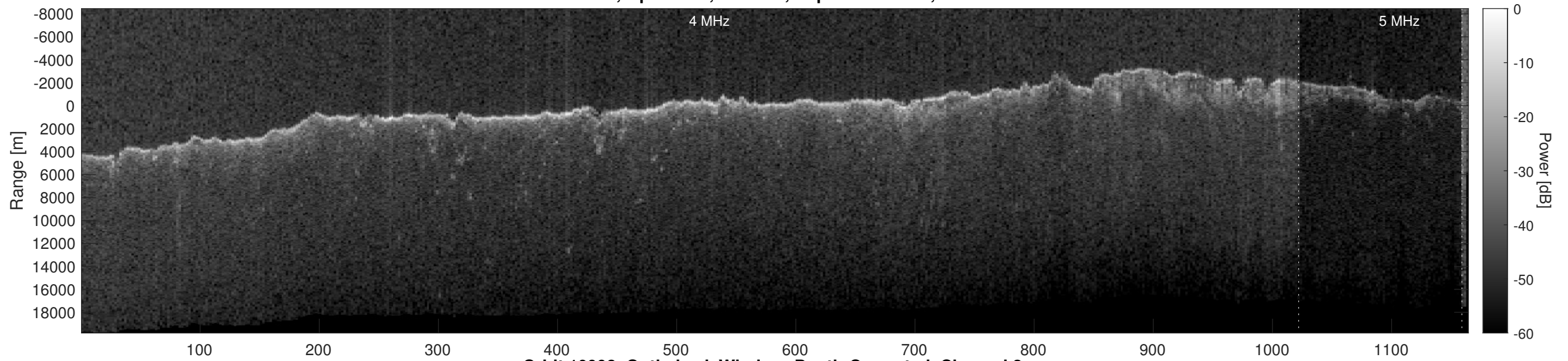
Orbit 10998, Optimized, Window, Depth-Corrected, Channel 2
