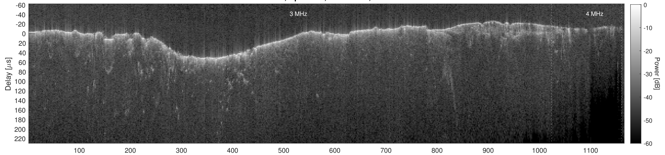
Orbit 11001, Cluttergram
