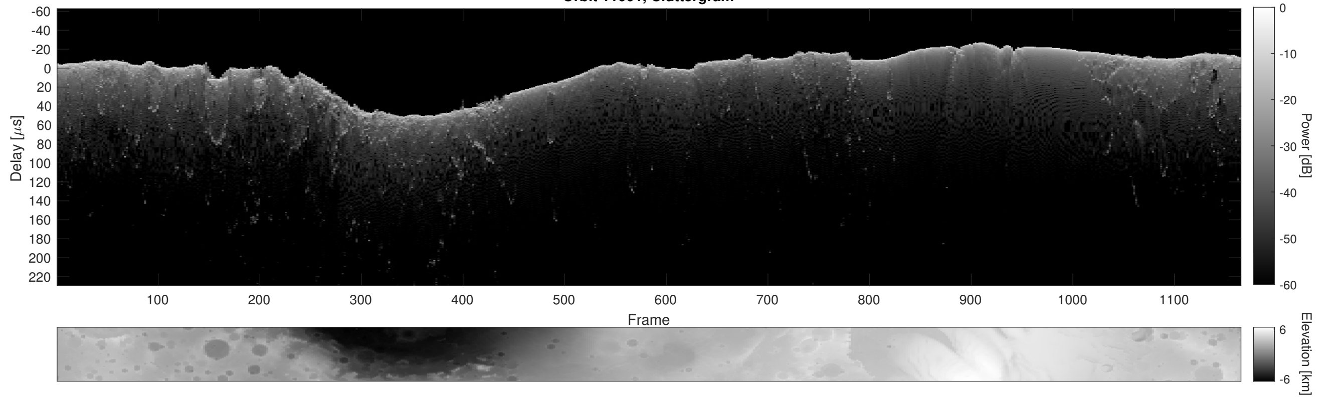
Orbit 11001, Cluttergram
