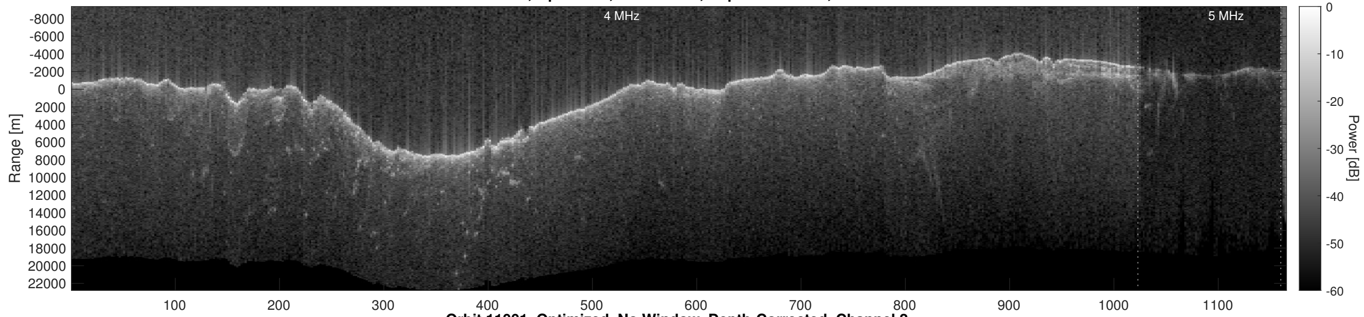
Orbit 11001, Optimized, No Window, Depth-Corrected, Channel 2
