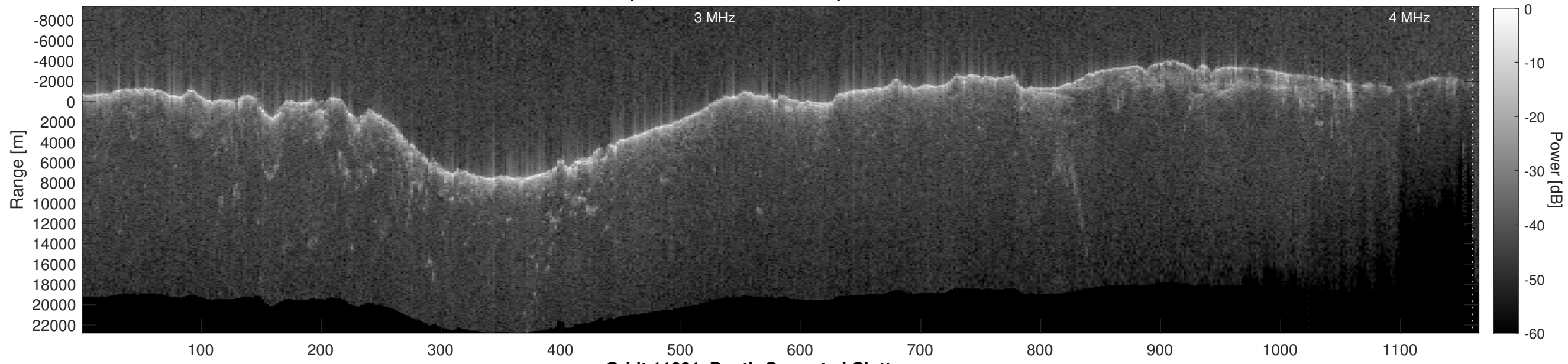
Orbit 11001, Depth-Corrected Cluttergram
