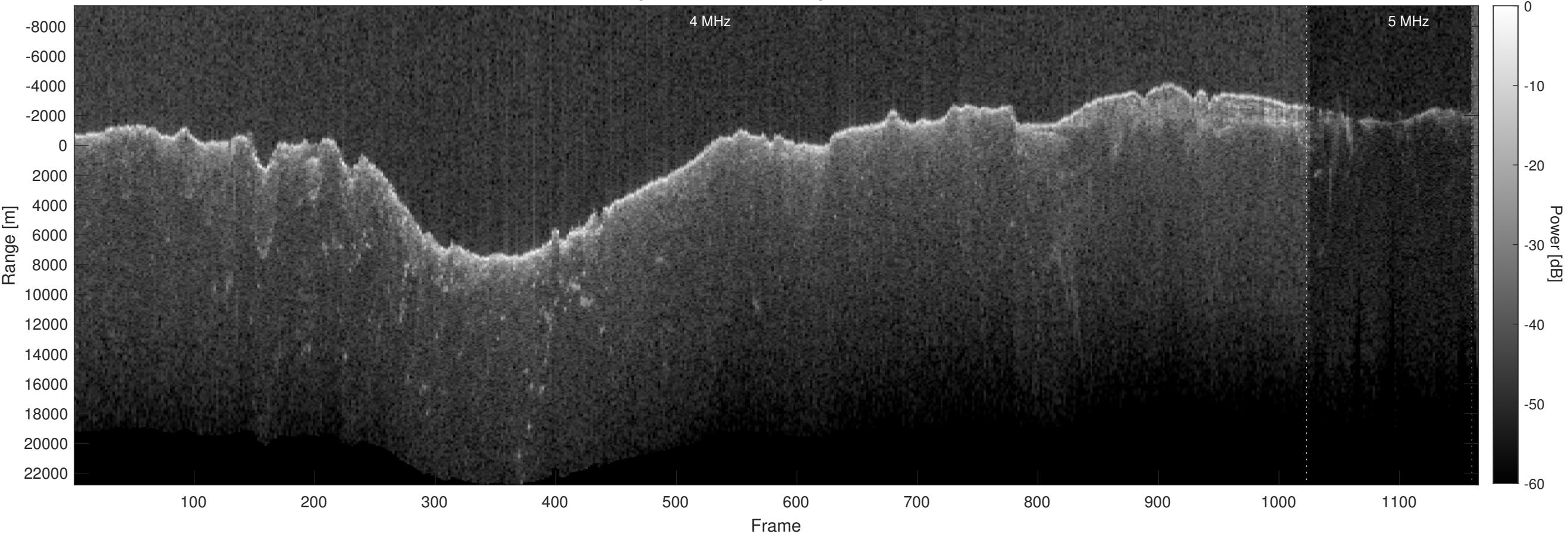
Orbit 11001, Optimized, Window, Depth-Corrected, Channel 2
