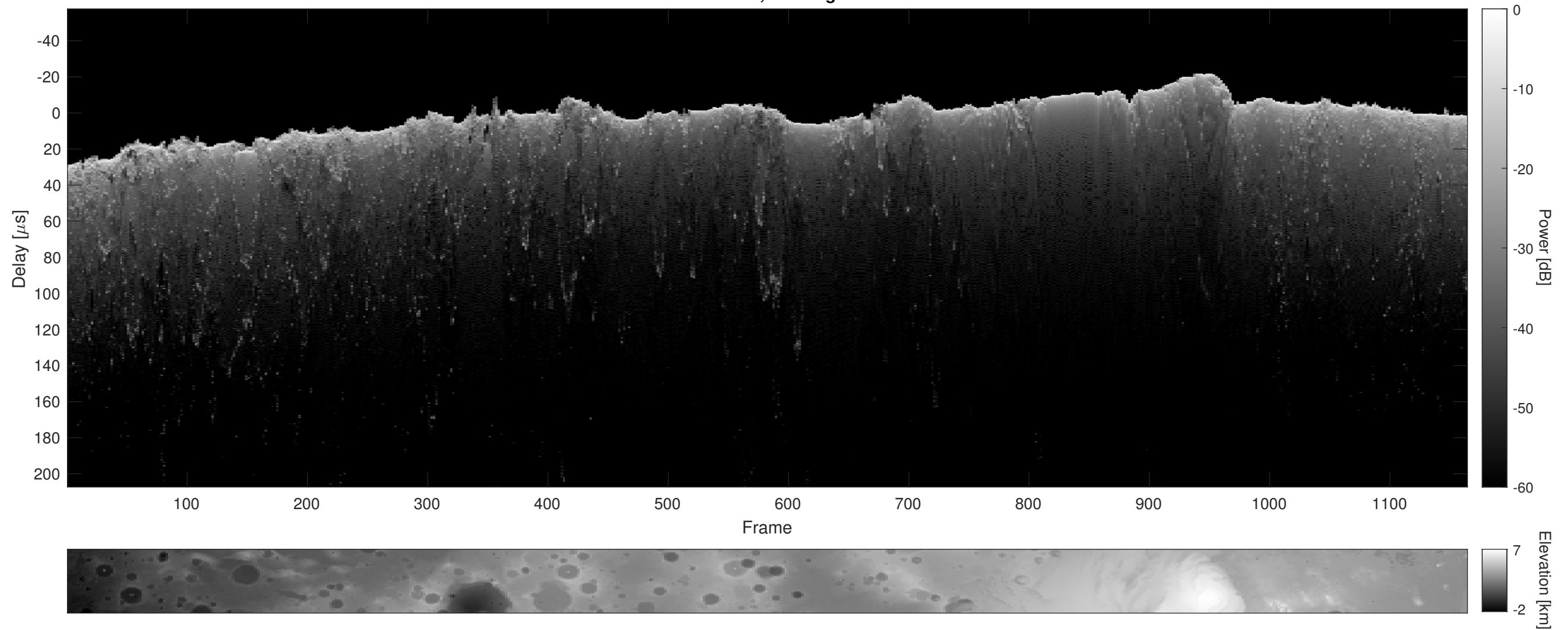
Orbit 11003, Cluttergram
