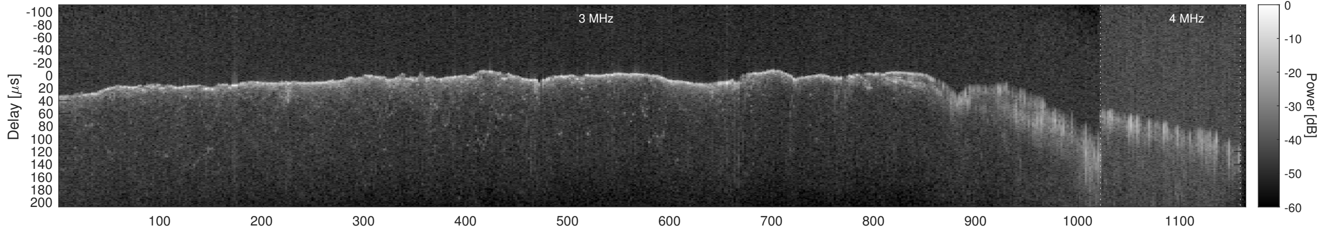
Orbit 11003, Window, Channel 2, Chapman
