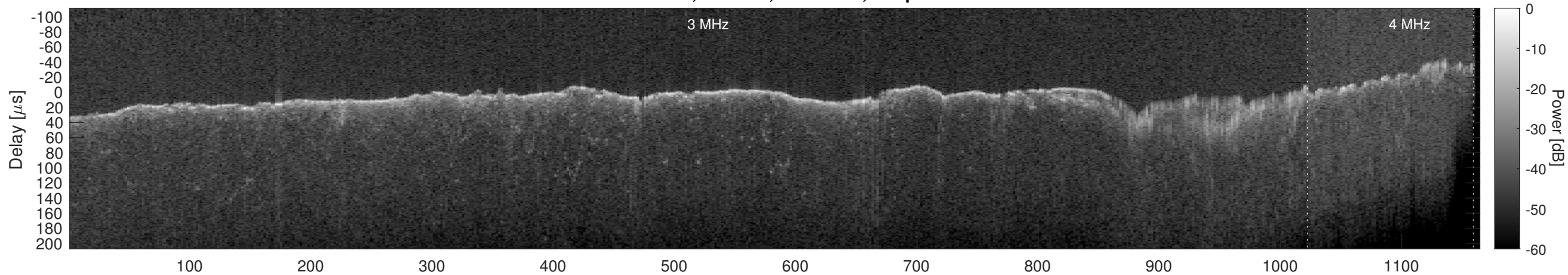
Orbit 11003, Window, Channel 2, Optimized
