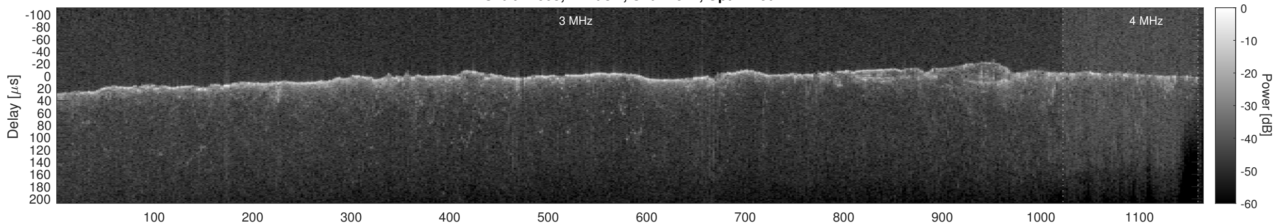
Orbit 11003, Cluttergram
