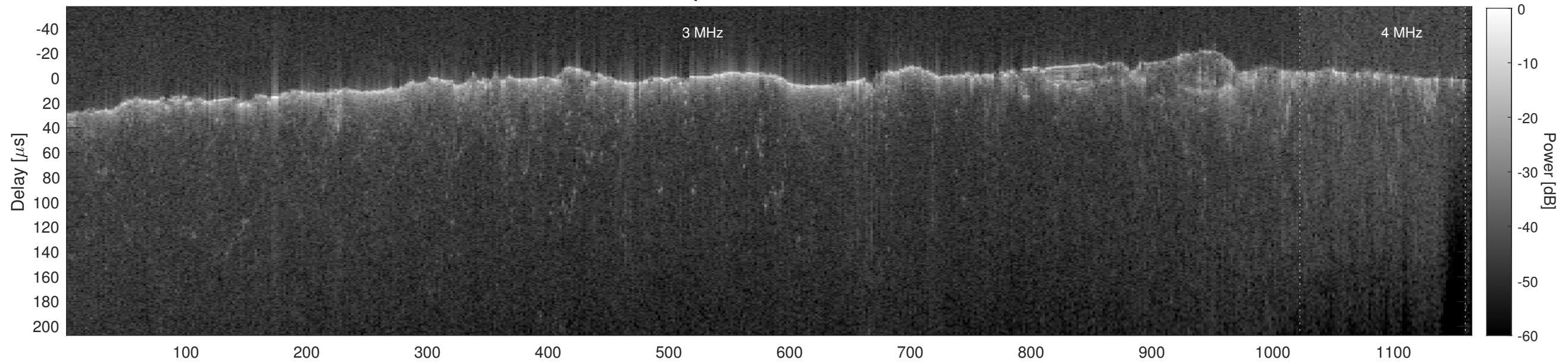
Orbit 11003, Cluttergram
