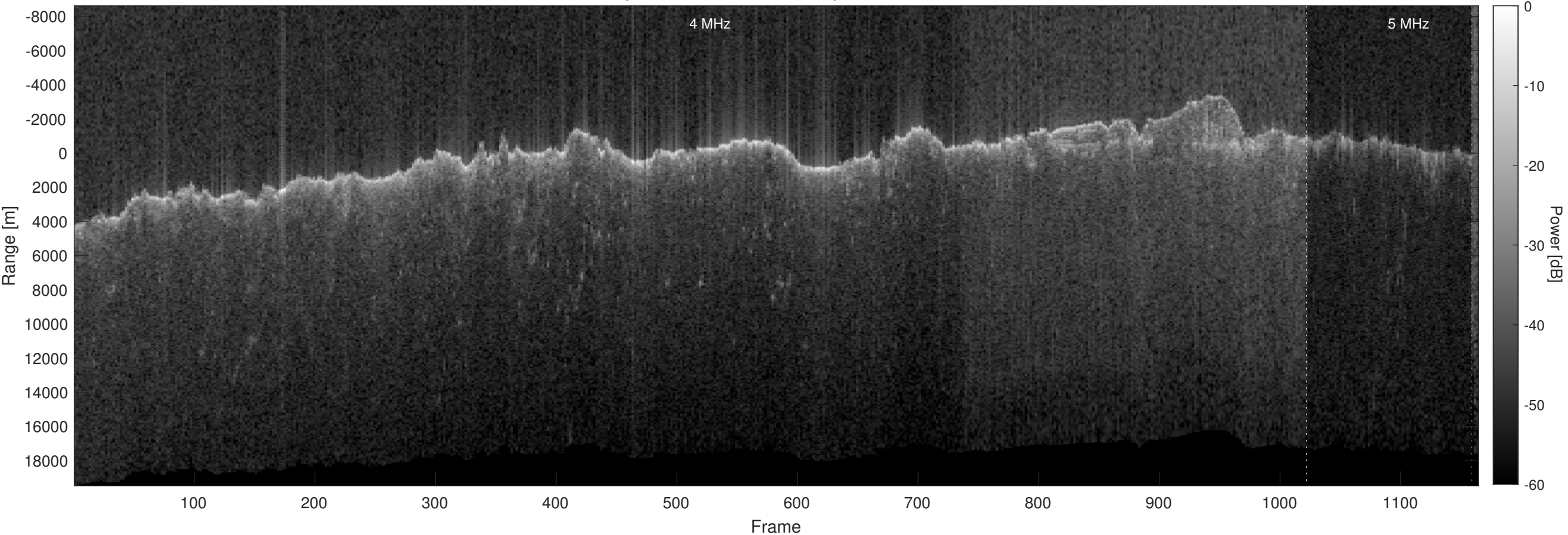
Orbit 11003, Optimized, No Window, Depth-Corrected, Channel 2
