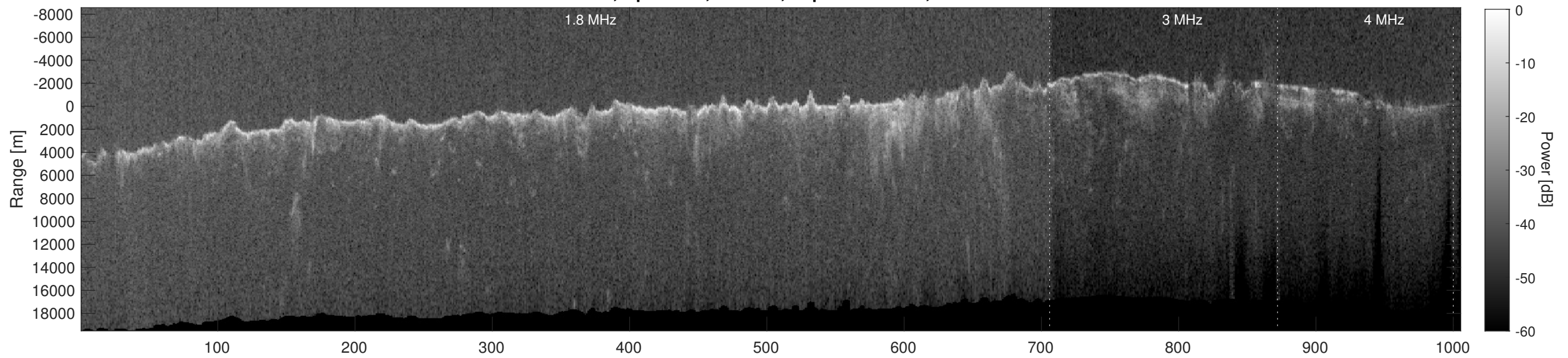
Orbit 11005, Depth-Corrected Cluttergram
