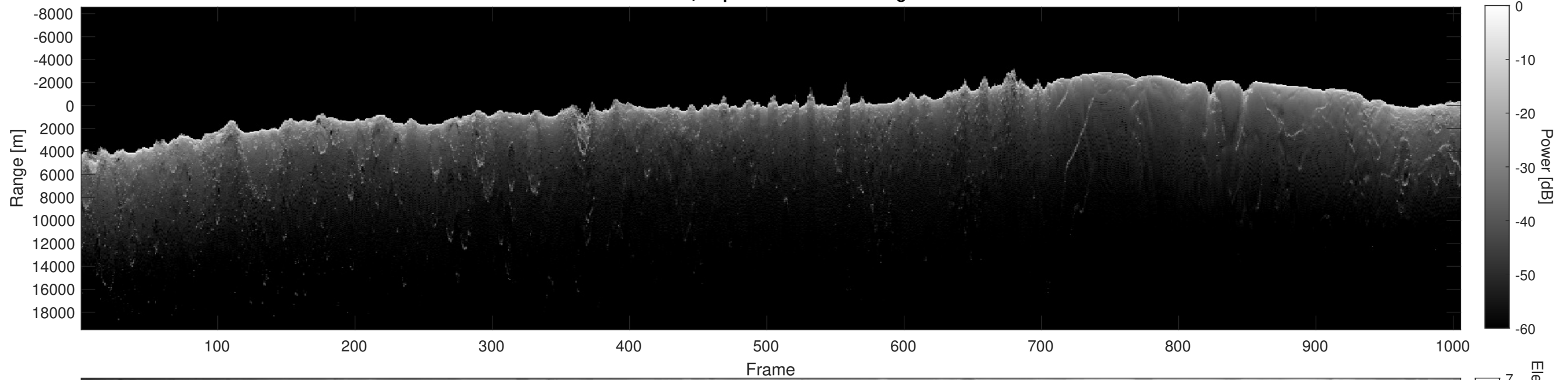
Orbit 11005, Depth-Corrected Cluttergram
