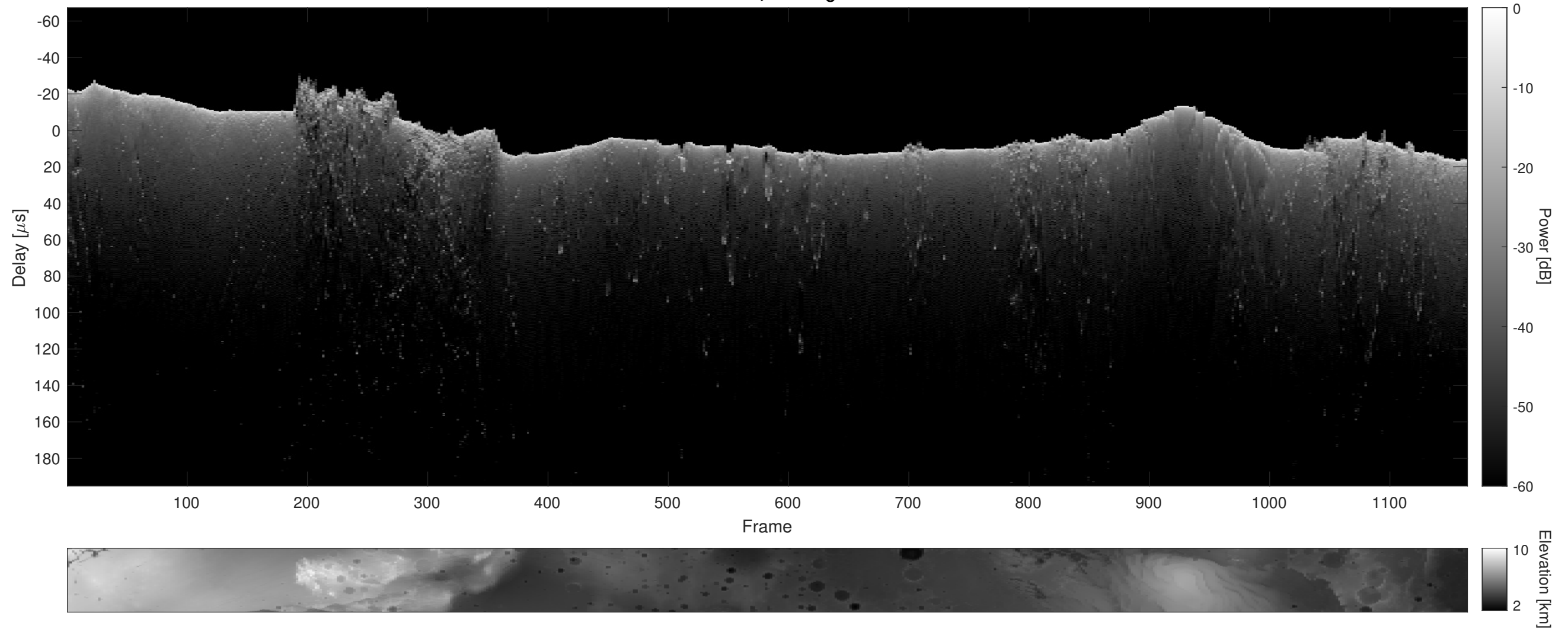
Orbit 11006, Cluttergram
