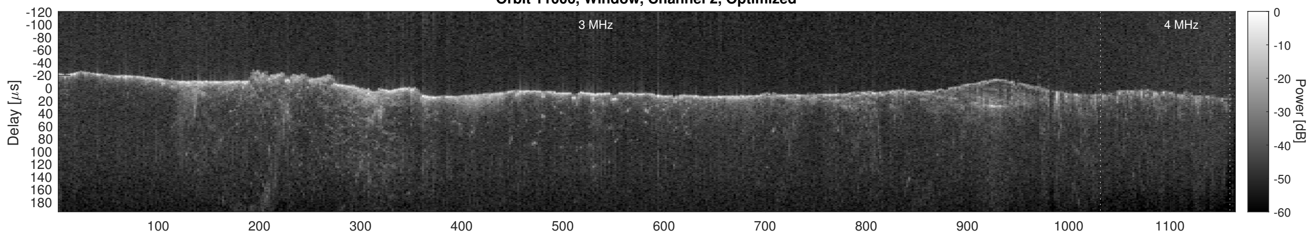
Orbit 11006, Cluttergram
