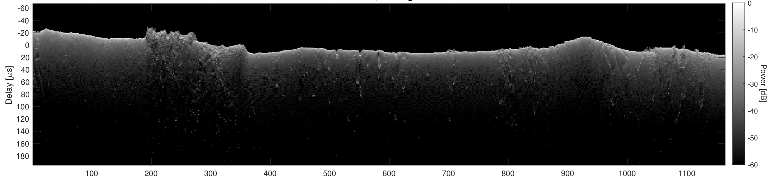
Orbit 11006, Cluttergram
