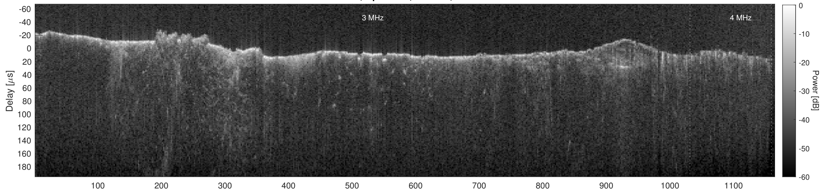
Orbit 11006, Cluttergram
