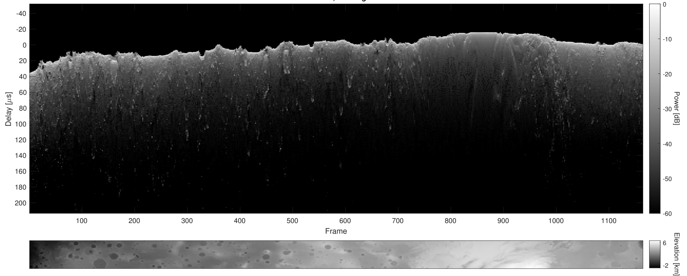
Orbit 11007, Cluttergram
