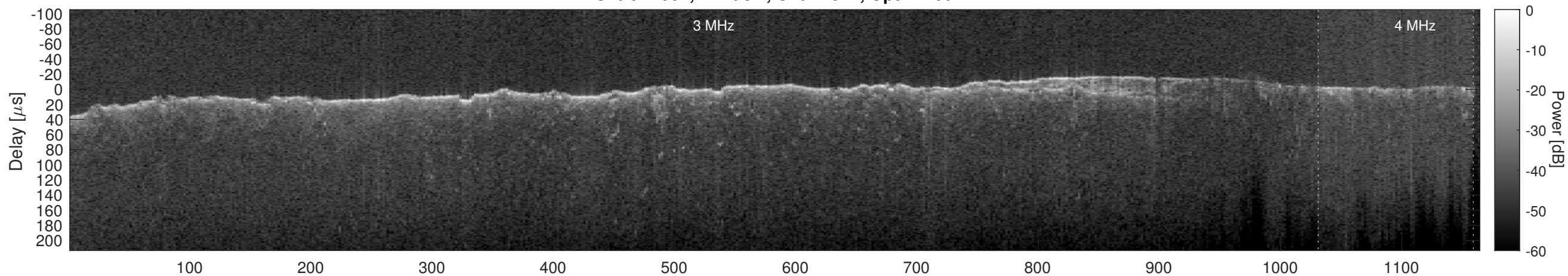
Orbit 11007, Cluttergram
