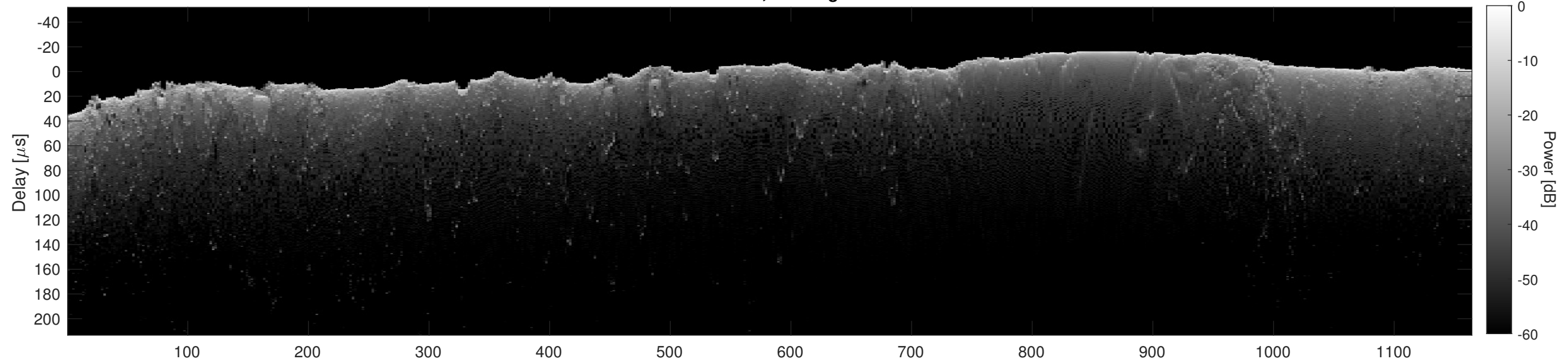
Orbit 11007, Cluttergram
