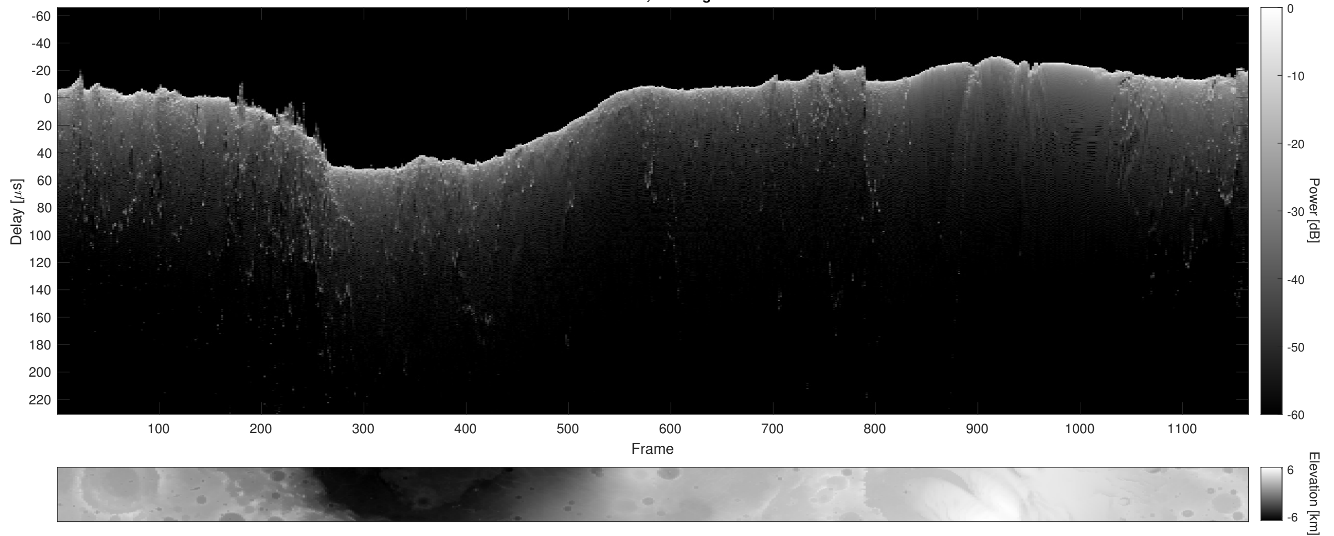
Orbit 11008, Cluttergram
