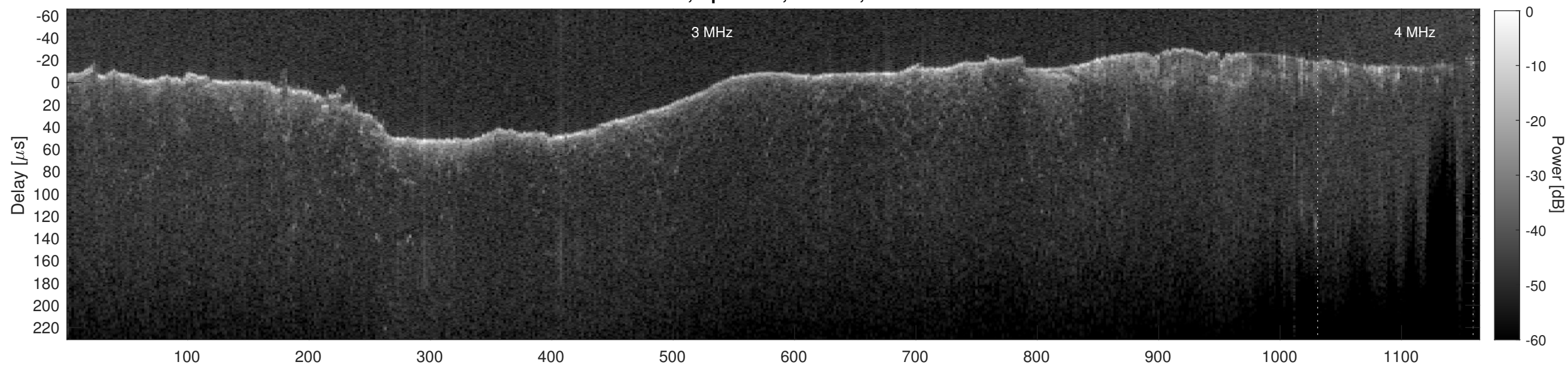
Orbit 11008, Cluttergram
