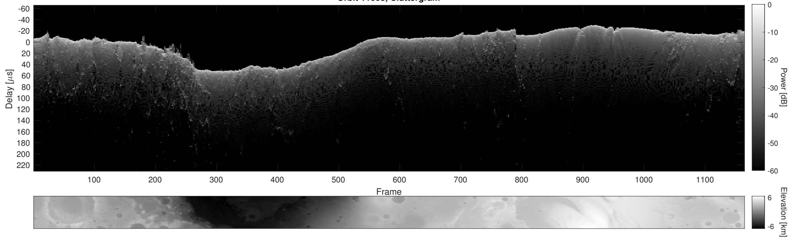
Orbit 11008, Cluttergram
