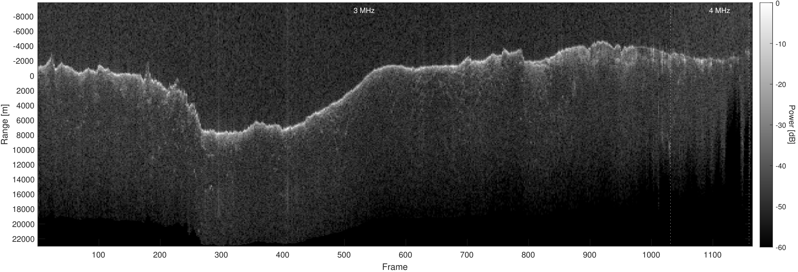
Orbit 11008, Optimized, Window, Depth-Corrected, Channel 2
