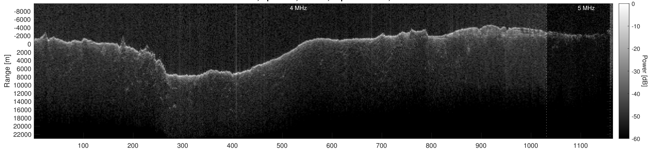
Orbit 11008, Optimized, Window, Depth-Corrected, Channel 2
