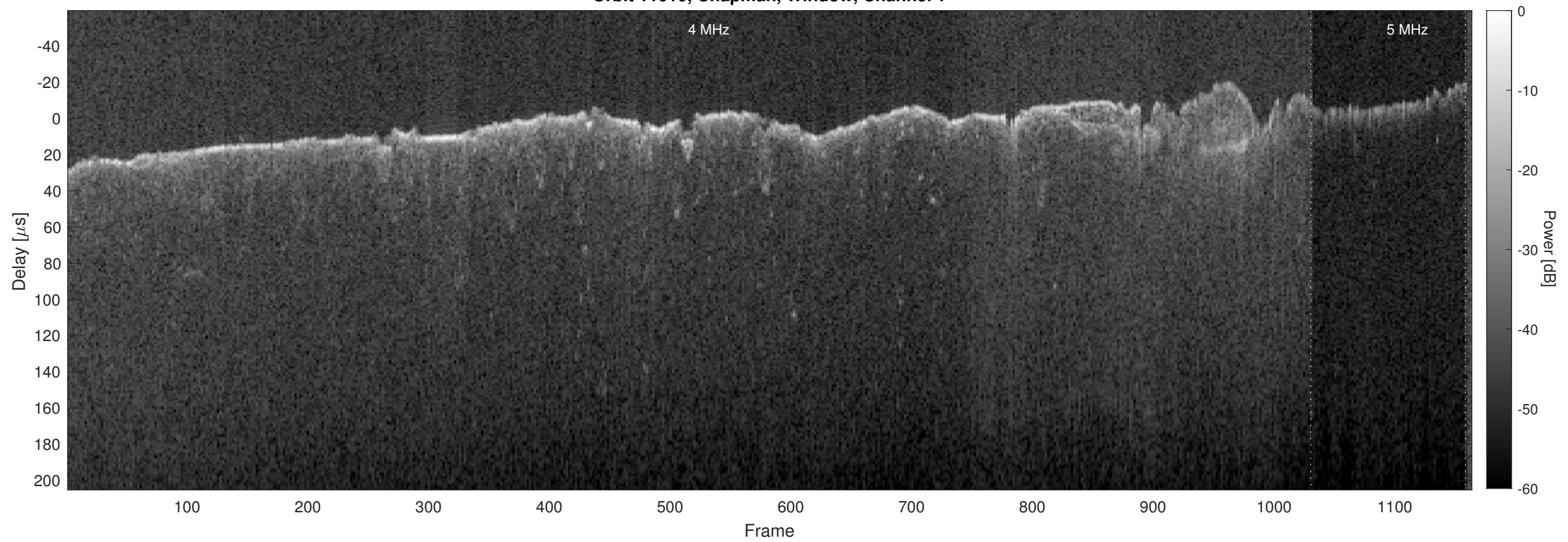
Orbit 11010, Chapman, Window, Channel 2
