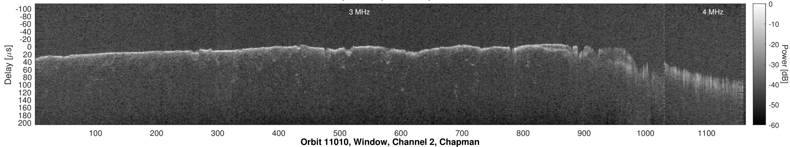
Orbit 11010, Window, Channel 2, Uncorrected
