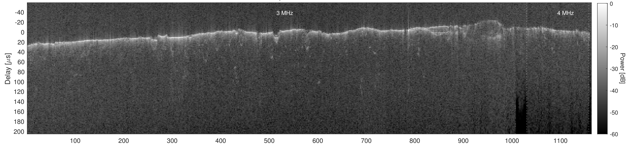
Orbit 11010, Cluttergram
