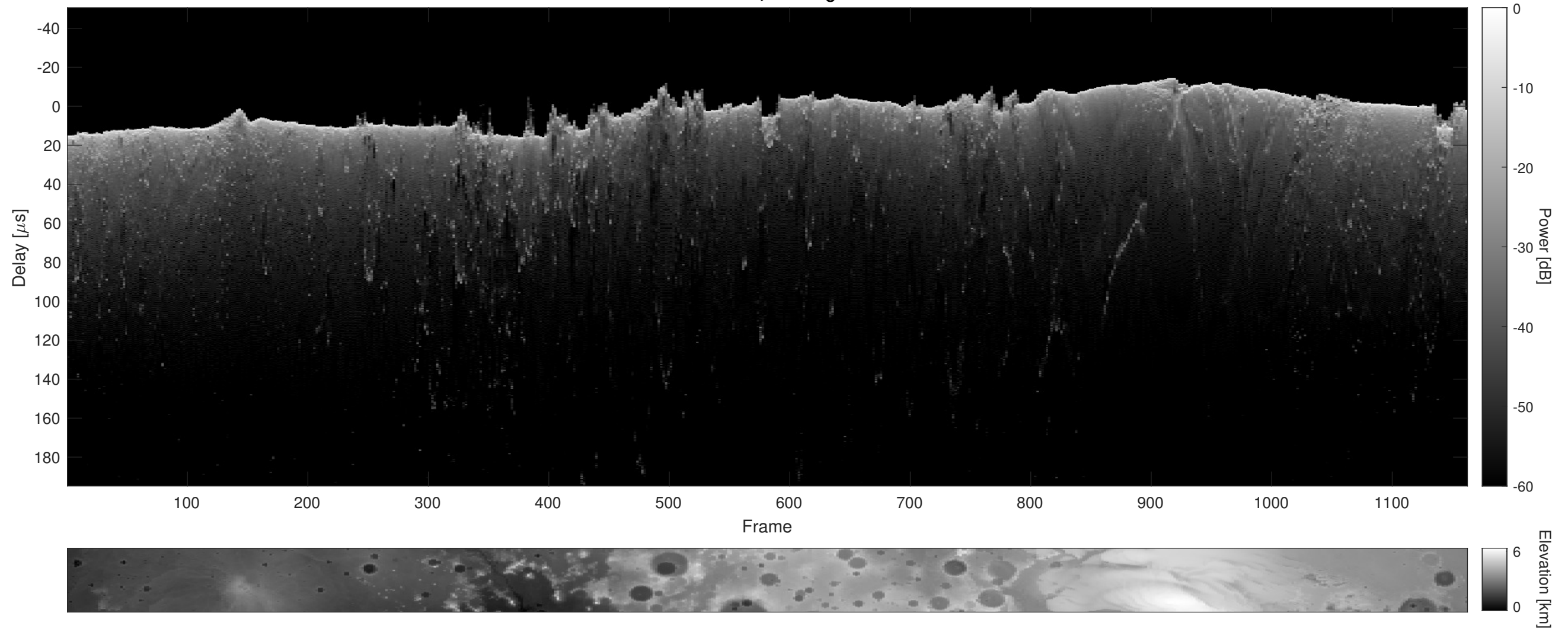
Orbit 11011, Cluttergram
