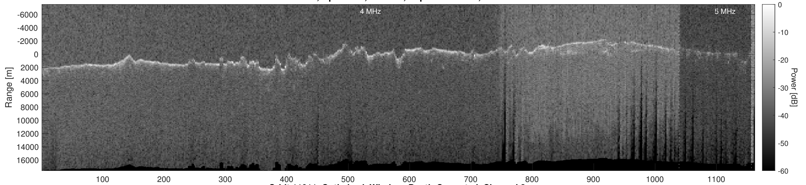
Orbit 11011, Optimized, Window, Depth-Corrected, Channel 2
