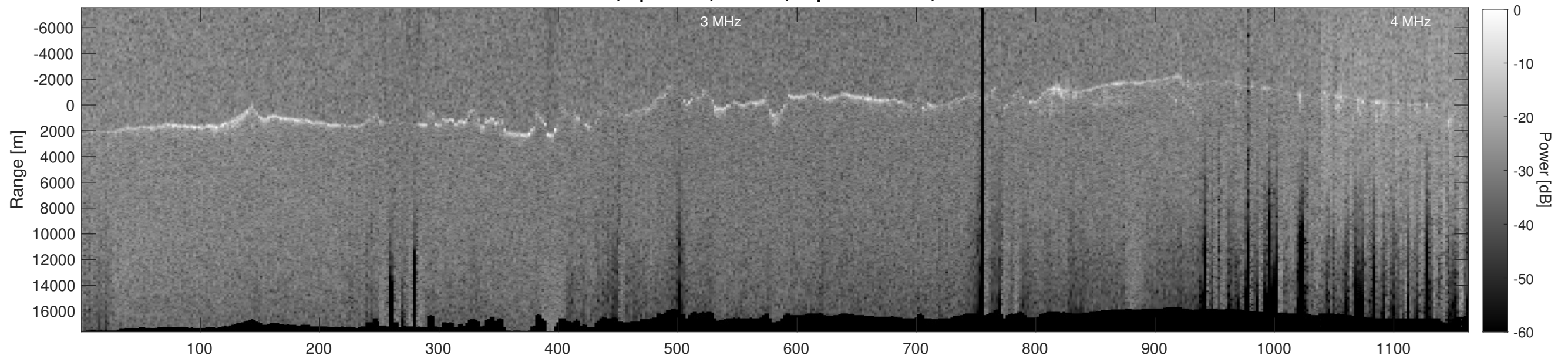
Orbit 11011, Depth-Corrected Cluttergram
