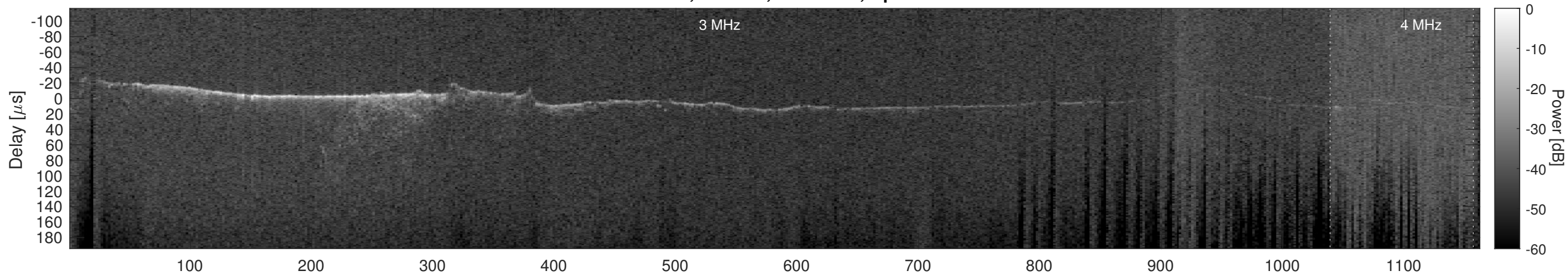
Orbit 11013, Cluttergram
