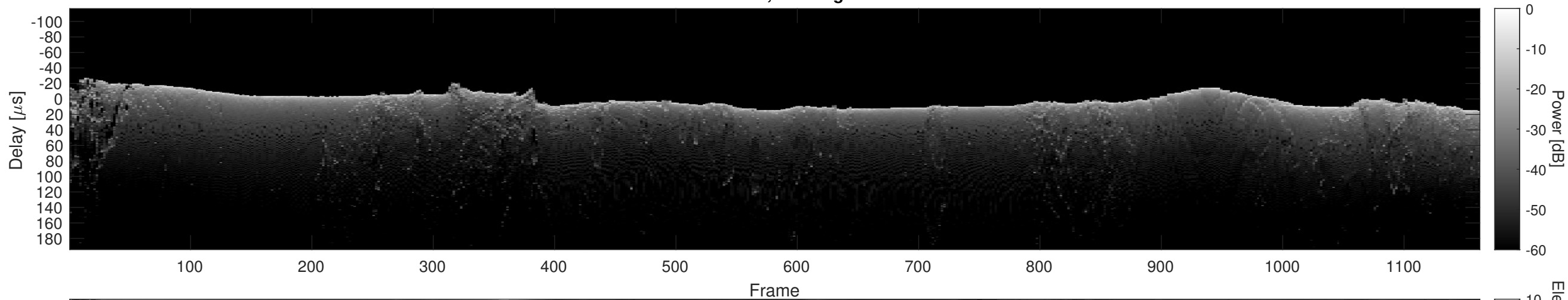
Orbit 11013, Cluttergram
