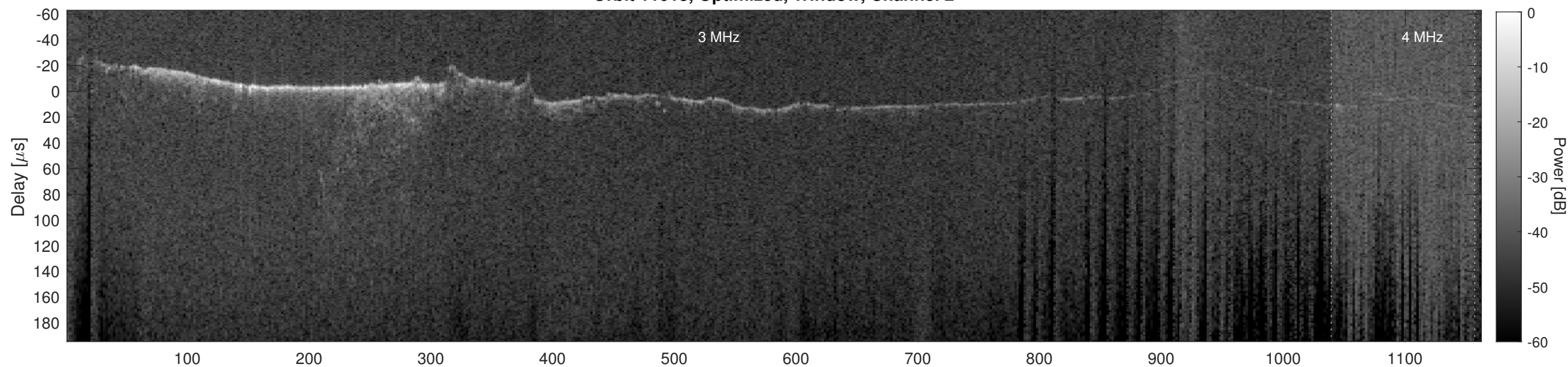
Orbit 11013, Cluttergram
