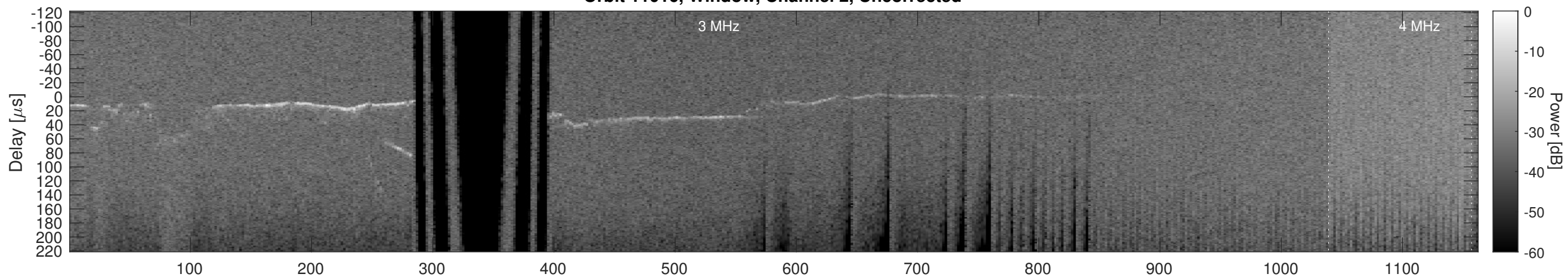
Orbit 11016, Window, Channel 2, Chapman
