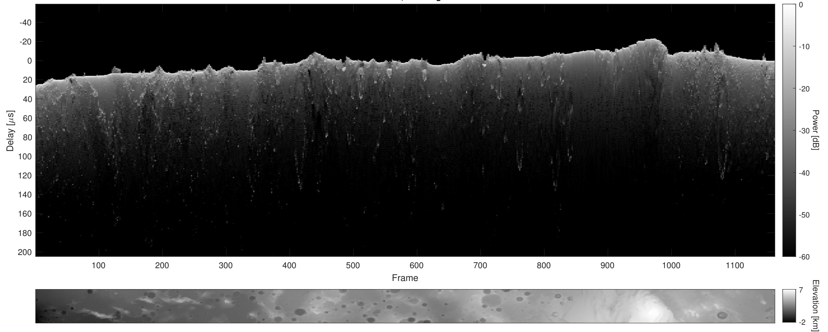
Orbit 11017, Cluttergram
