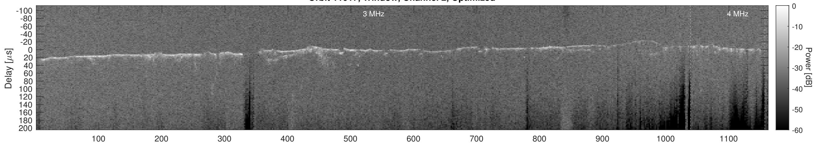
Orbit 11017, Cluttergram
