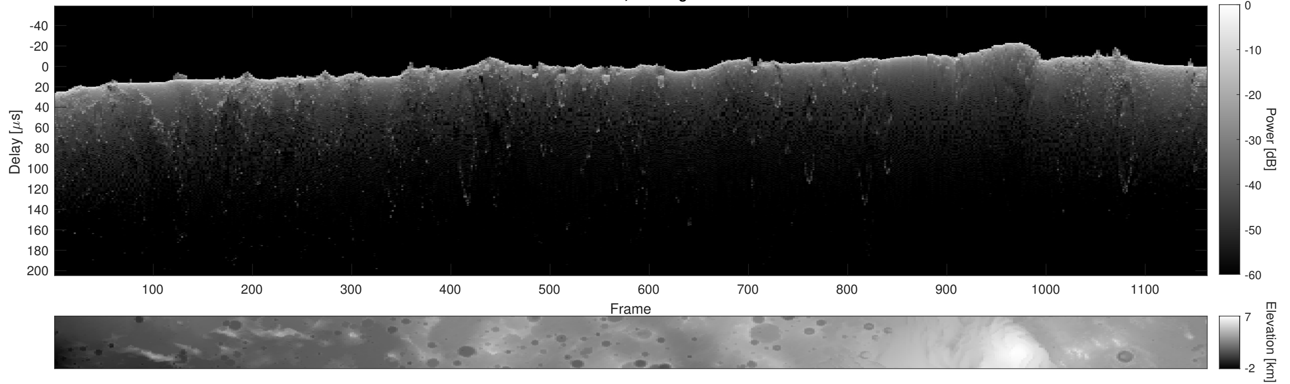
Orbit 11017, Cluttergram
