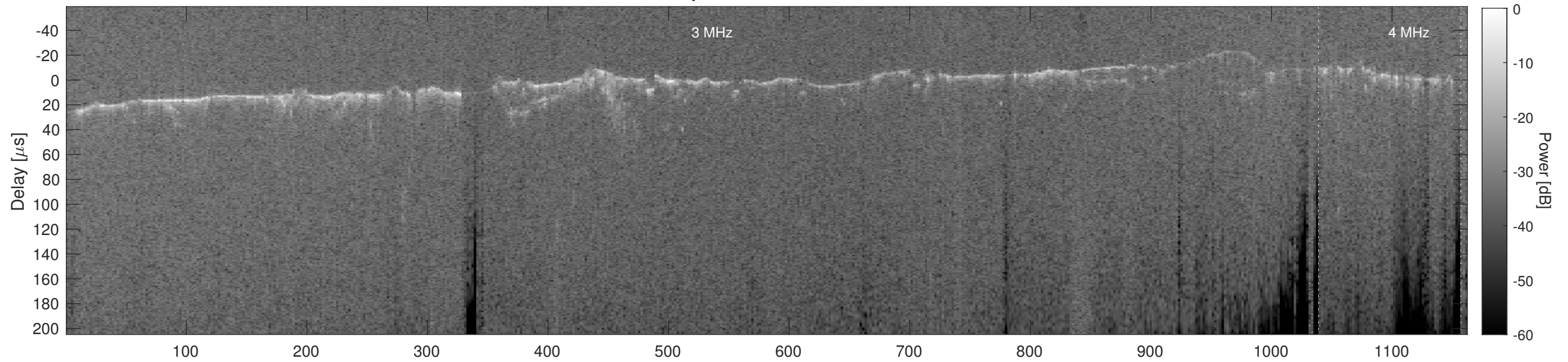
Orbit 11017, Cluttergram
