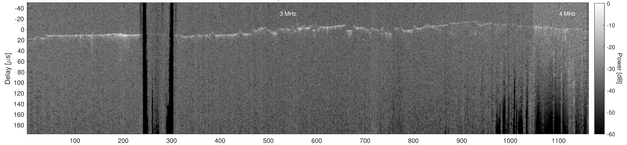
Orbit 11018, Cluttergram
