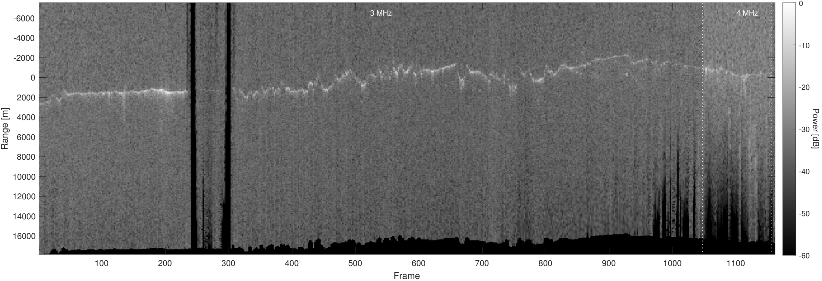
Orbit 11018, Optimized, No Window, Depth-Corrected, Channel 2
