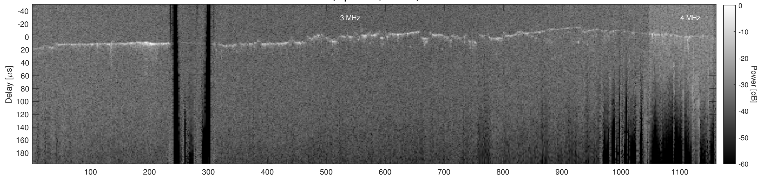
Orbit 11018, Cluttergram
