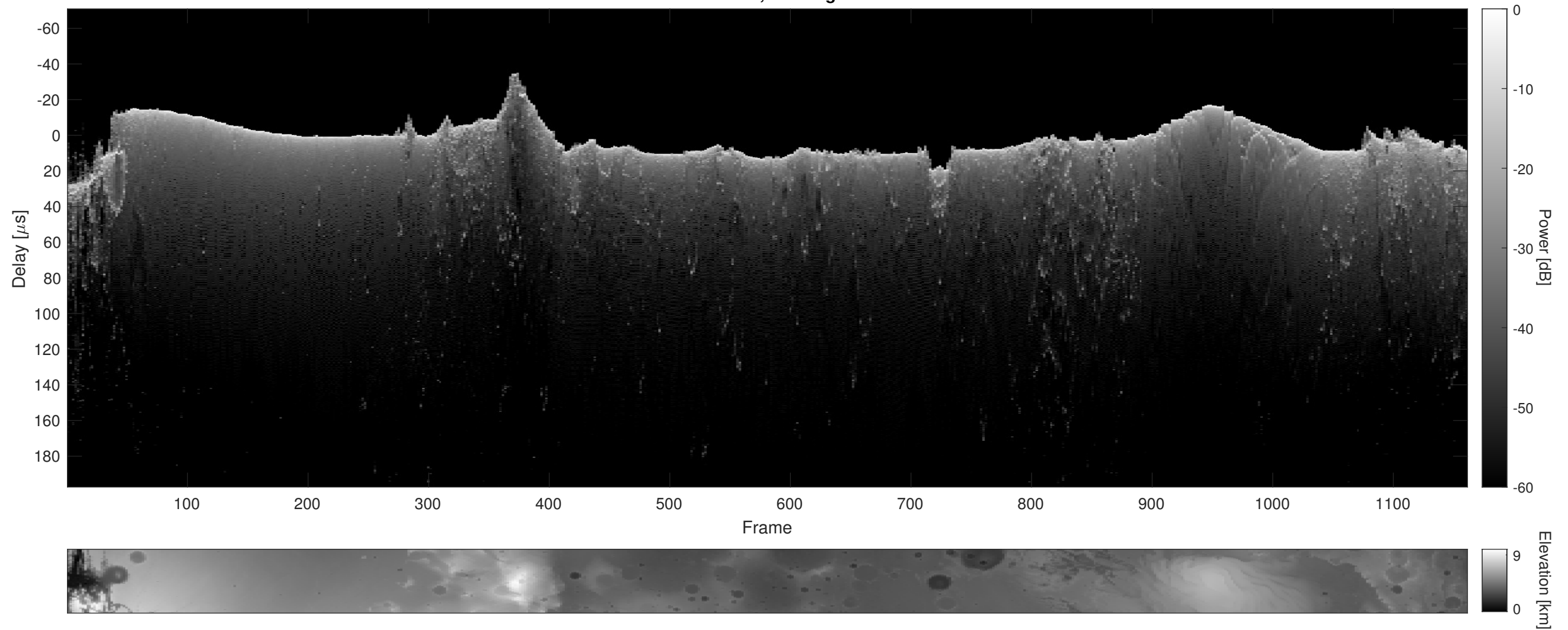
Orbit 11020, Cluttergram
