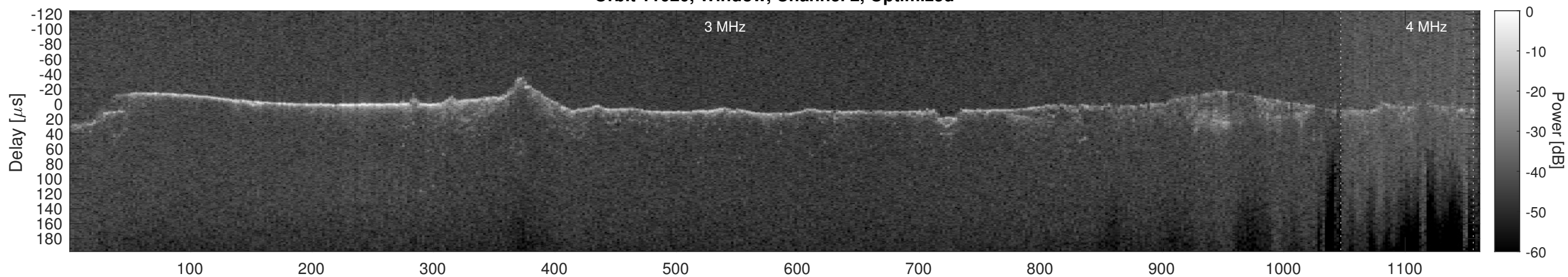
Orbit 11020, Cluttergram
