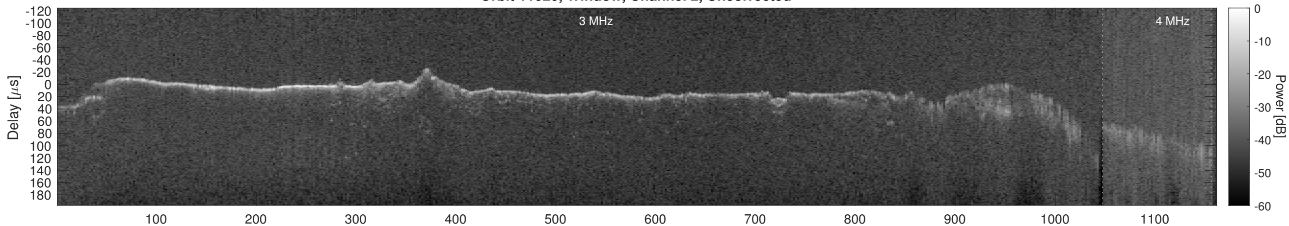
Orbit 11020, Window, Channel 2, Chapman
