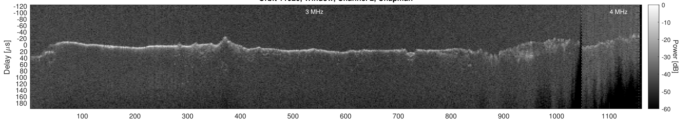
Orbit 11020, Window, Channel 2, Optimized
