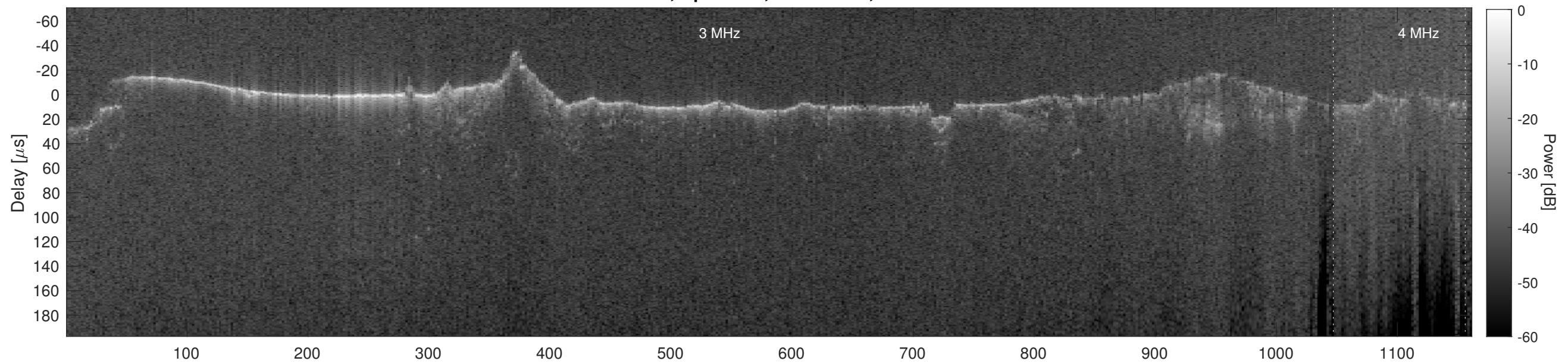
Orbit 11020, Cluttergram
