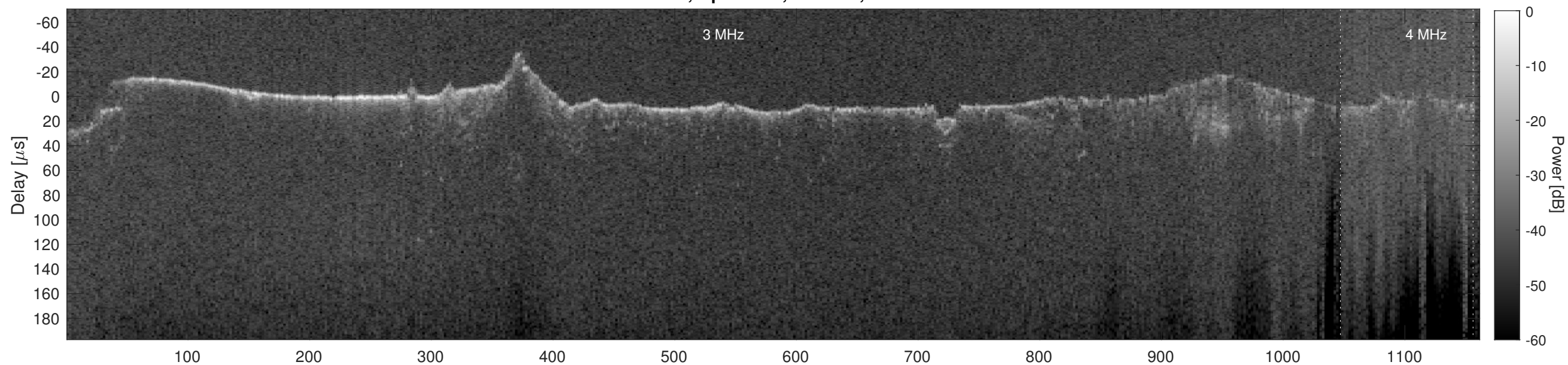
Orbit 11020, Cluttergram
