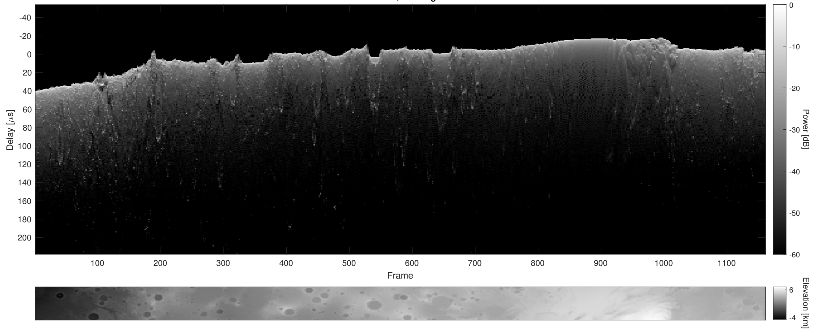
Orbit 11021, Cluttergram
